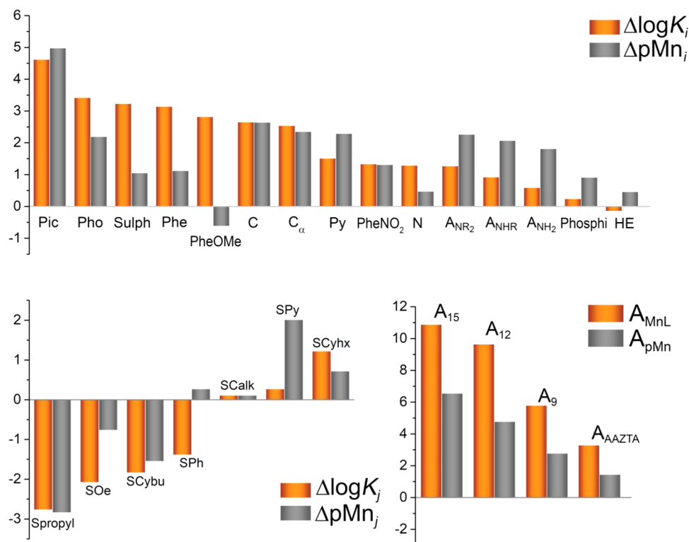
Figure 3. Comparison of the contributions of the different structural descriptors to \log K_{\text{MnL}} and \text{pMn} , obtained from the least-squares fit of the stability data to eqs 1 and 2. Structural descriptors detailed in Table 3.
