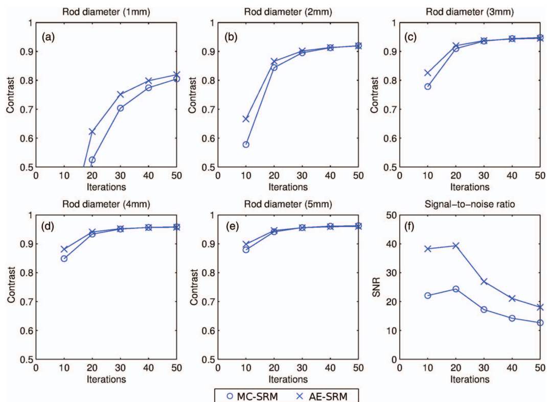
FIG. 4. Contrast versus number of iterations for the different cylinder diameters (a)–(e), obtained from reconstructed images by using MC-SRM and AE-SRM. SNR versus number of iterations from reconstructed images by using MC-SRM and AE-SRM (f).
