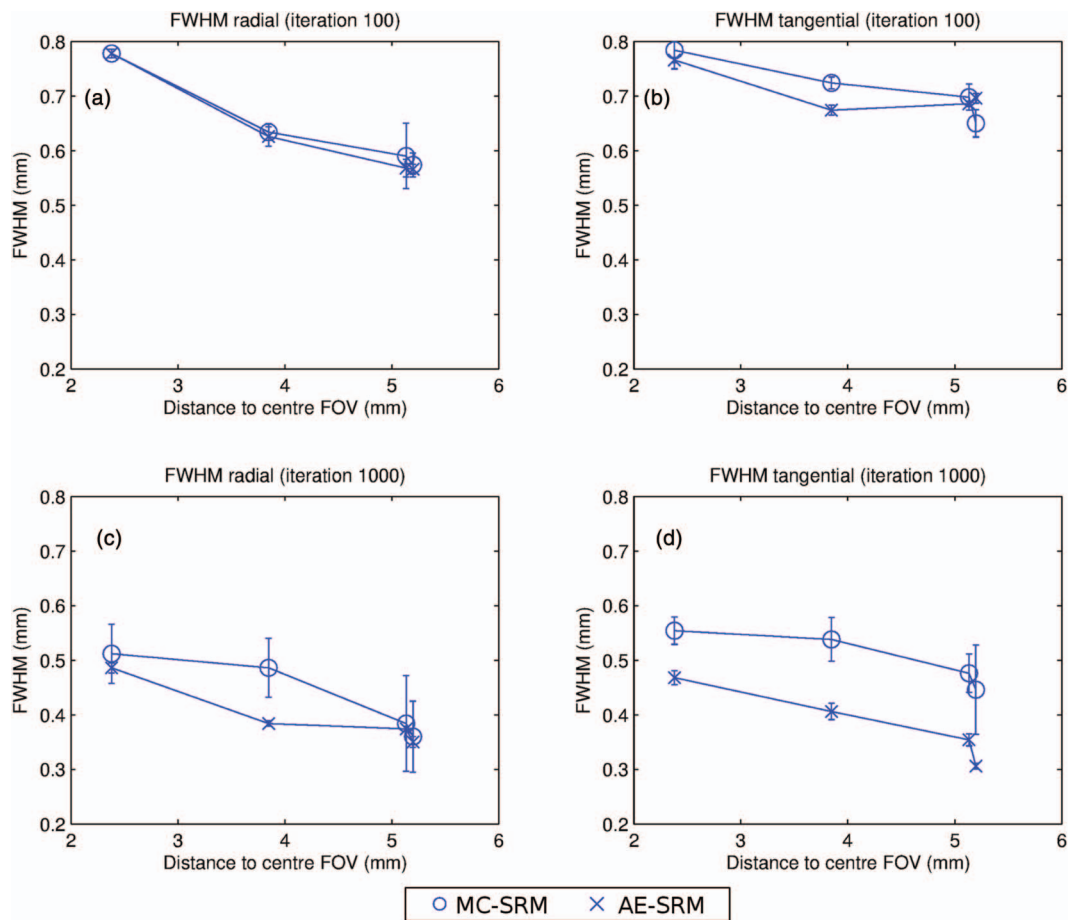
FIG. 6. Radial (left) and tangential (right) spatial resolution for rods placed at different distances from the center FOV (iteration 100 and 1000). The rods are placed at distances from the center FOV of 2.3, 3.8, 5.1, and 5.2 mm.
