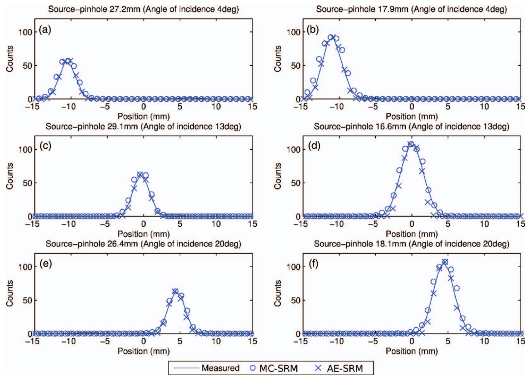
FIG. 2. PSFs for point sources placed at distances greater (27.2, 29.1, and 26.4 mm) and smaller (17.9, 16.6, and 18.1 mm) than the radius of rotation, and for three incidence angles ( 4^\circ , 13^\circ , and 20^\circ ). The transverse profiles were obtained through projected points using MC-SRM and AE-SRM. Experimental profiles are also shown for comparison.
