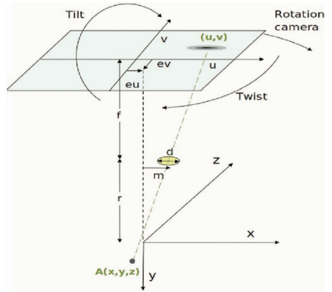
FIG. 1. Rotating-camera geometry, where z axis is the rotation axis of the system, and A(x, y, z) is the activity distribution defined in the xyz system and projected into the uv system through the pinhole ( d diameter).
